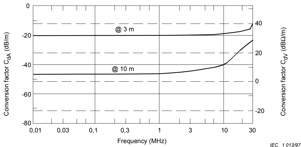
Figure C.10 – Conversion factors C_{dA} (for conversion into dB (μA/m)) and C_{dV} (for conversion into dB (μV/m)) for two standardized measuring distances d
