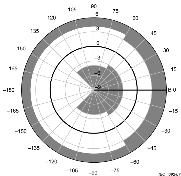
Figure 16b – 6 GHz to 18 GHz
