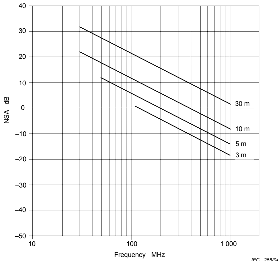
Figure 7 – Graph of theoretical free-space NSA as a function of the frequency for different measurement distances (see Equation 4)
