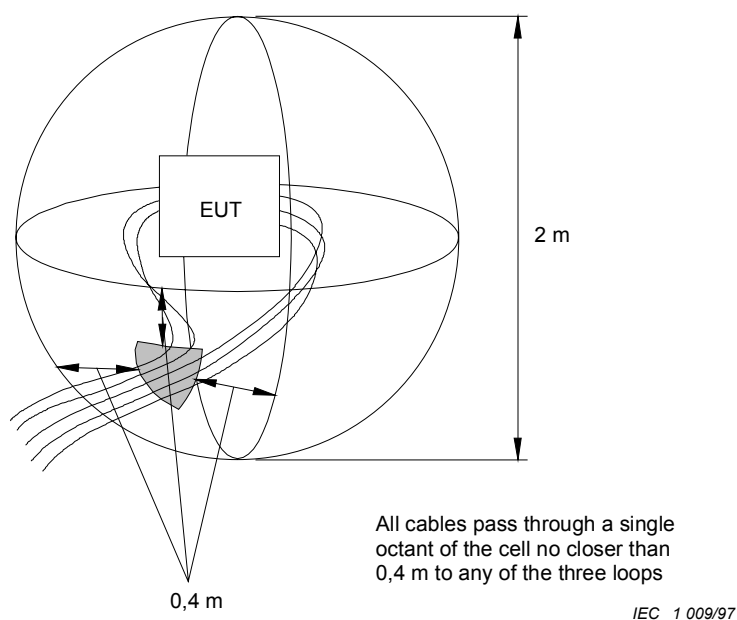
Figure C.6 – Example showing the routing of several cables from an EUT to ensure that there is no capacitive coupling from the leads to the loop
